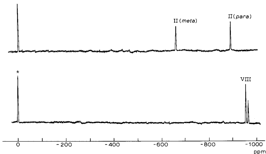
Fig. 1. ^{195}\text{Pt} NMR spectra of complexes II and VIII in acetone solutions. * Reference: \text{Na}_2\text{PtCl}_6 \cdot 6\text{H}_2\text{O} ( \delta = 0 ppm).
