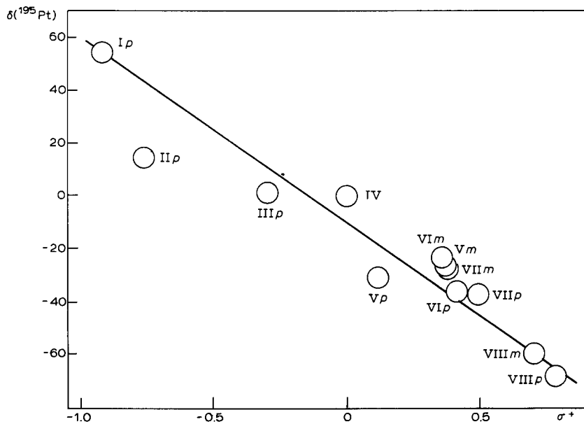
Fig. 3. Plot of the ^{195}\text{Pt} chemical shifts \delta of complexes I–VIII versus Brown's \sigma^+ -constants.
