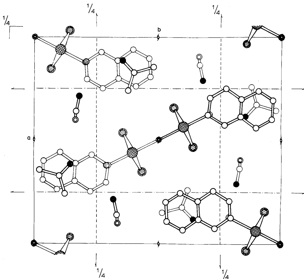
Fig. 1. The crystal structure of complex I projected along the c -axis:
