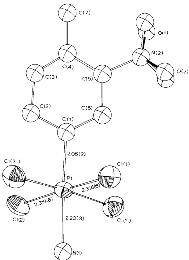
Fig. 3. The molecular structure of complex II (configuration and some important interatomic distances, Å).
