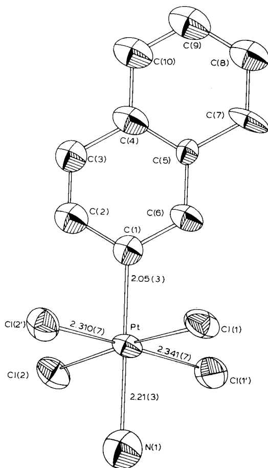
Fig. 2. The molecular structure of complex I (configuration and some important interatomic distances, Å).
