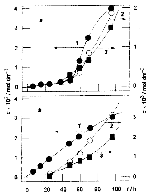
Fig. 1 Accumulation of cyclooctyl hydroperoxide (curves 1), cyclooctanone (2) and cyclooctanol (3) in the oxidations of cyclooctane (0.15 mol/dm 3 ) with H 2 O 2 (0.45 mol/dm 3 ) in acetonitrile at 70°C catalysed by Ni(ClO 4 ) 2 (5 × 10 -4 mol/dm 3 ) in the absence (graph a) and in the presence of TMTACN (0.0012 mol/dm 3 ) (b).
