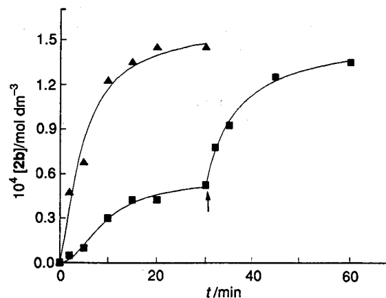
Fig. 2 Accumulation of complex 2b during irradiation (light source as in Fig. 1, \lambda = 600 \text{ nm} ) of an acetone solution of complex 1b ( 3 \times 10^{-4} \text{ mol dm}^{-3} ) in air ( \blacktriangle ) or in a \text{N}_2 atmosphere in acetone distilled under \text{N}_2 before irradiation ( \blacksquare ). The arrow indicates when a pulse of air was bubbled through the solution
