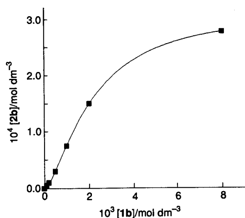
Fig. 3 Plot of concentration of complex 2b after 2 min irradiation (light source as in Fig. 1) versus initial concentration of complex 1b , dried acetone solutions
