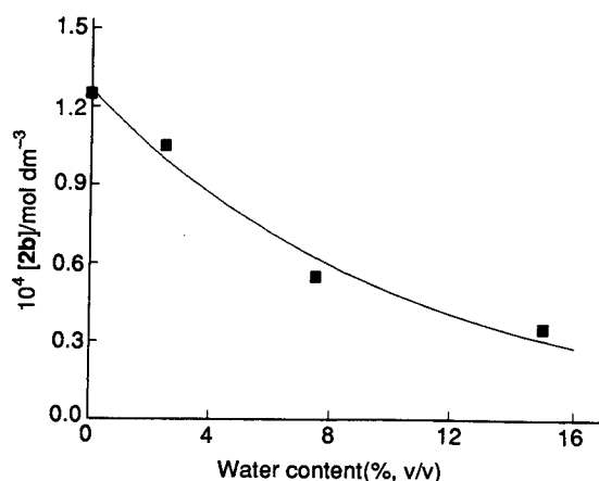
Fig. 6 Plot of concentration of complex 2b after 5 min of irradiation ('Osram Ultra Vitalux' lamp) of an acetone solution of complex 1b ( 5 \times 10^{-4} mol \text{dm}^{-3} ) versus the water content (% v/v)
