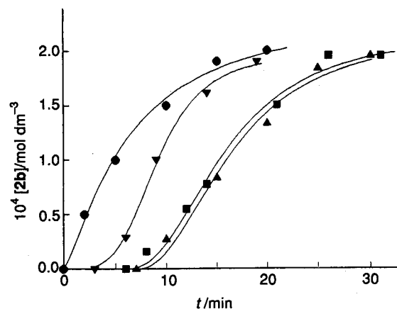
Fig. 4 Accumulation of complex 2b during irradiation of an acetone solution of complex 1b ( 4 \times 10^{-4} mol dm ^{-3} ) by full light from an 'Osram Ultra Vitalux' lamp in the absence ( \bullet ) and in the presence of 4 \times 10^{-4} ( \nabla ), 8 \times 10^{-4} ( \blacksquare ) or 20 \times 10^{-4} ( \blacktriangle ) of PPh _3
