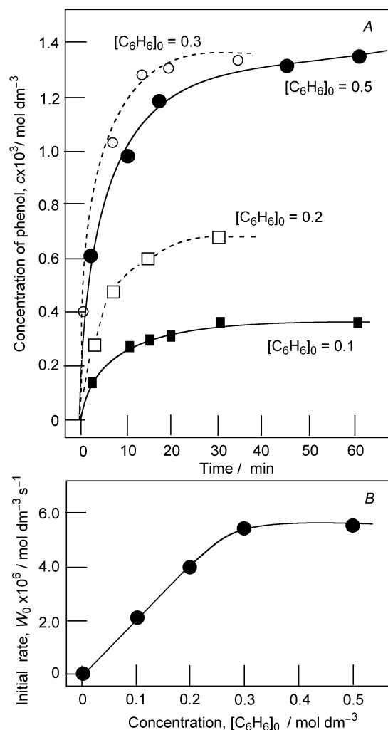
Figure 11. Reaction of benzene with \text{H}_2\text{O}_2 ( 0.04 \text{ mol dm}^{-3} ) catalyzed by \text{FeCl}_3 ( 5 \times 10^{-4} \text{ mol dm}^{-3} ) in MeCN at 25^\circ\text{C} . Graph A: accumulation of phenol with time at various initial concentrations of benzene ( \text{mol dm}^{-3} ). Graph B: plot of phenol accumulation initial rate measured from data of graph A versus initial concentration of benzene.
