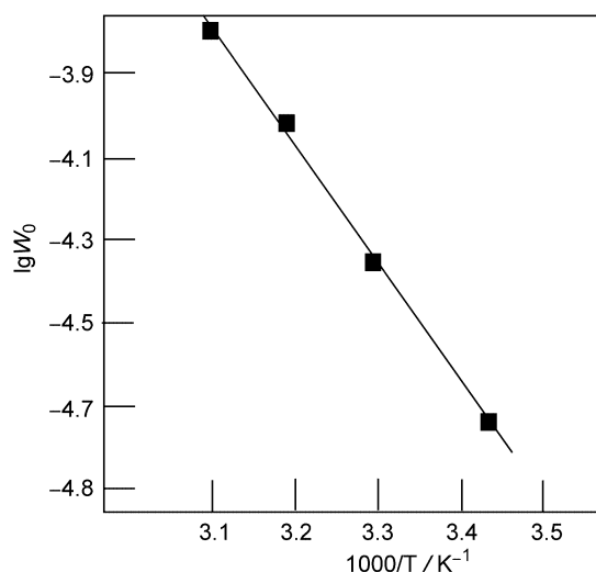
Figure 8. The Arrhenius plot for the cyclohexane (0.23 mol dm -3 ) oxygenation by H 2 O 2 (0.02 mol dm -3 ) in MeCN catalyzed by FeCl 3 (5 × 10 -4 mol dm -3 ) which corresponds the activation energy E a = 14 kcal mol -1 .
