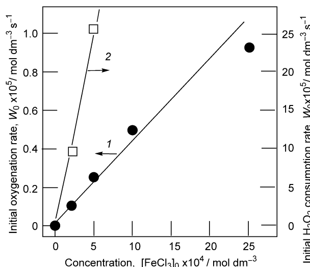
Figure 5. Cyclohexane oxidation with H 2 O 2 catalyzed by FeCl 3 : plot of dependence of the oxygenate accumulation initial rate (curve 1) and the H 2 O 2 consumption initial rate (curve 2) on initial FeCl 3 ·6 H 2 O concentration (at [cyclohexane] 0 = 0.46 mol dm -3 and [H 2 O 2 ] 0 = 0.05 mol dm -3 ) at 25 °C.
