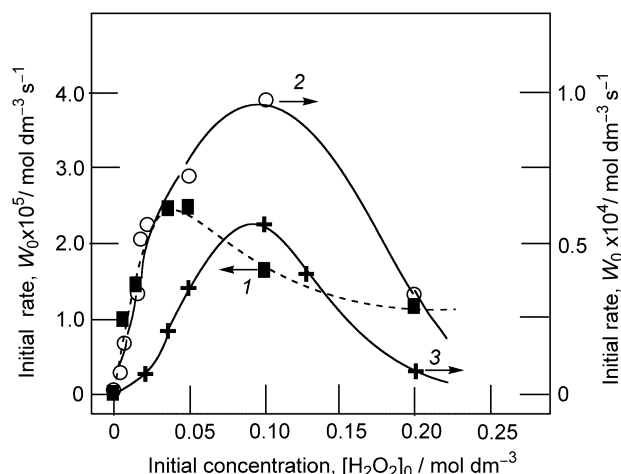
Figure 7. Decomposition of H 2 O 2 catalyzed by FeCl 3 ·6 H 2 O (5 × 10 -4 mol dm -3 ) in MeCN at 25 °C. Plots of initial rates of the cyclohexane oxygenates accumulation (curve 1) as well as (in the absence of cyclohexane) of H 2 O 2 consumption (curve 2), and O 2 evolution (curve 3) versus initial H 2 O 2 concentration are shown.
